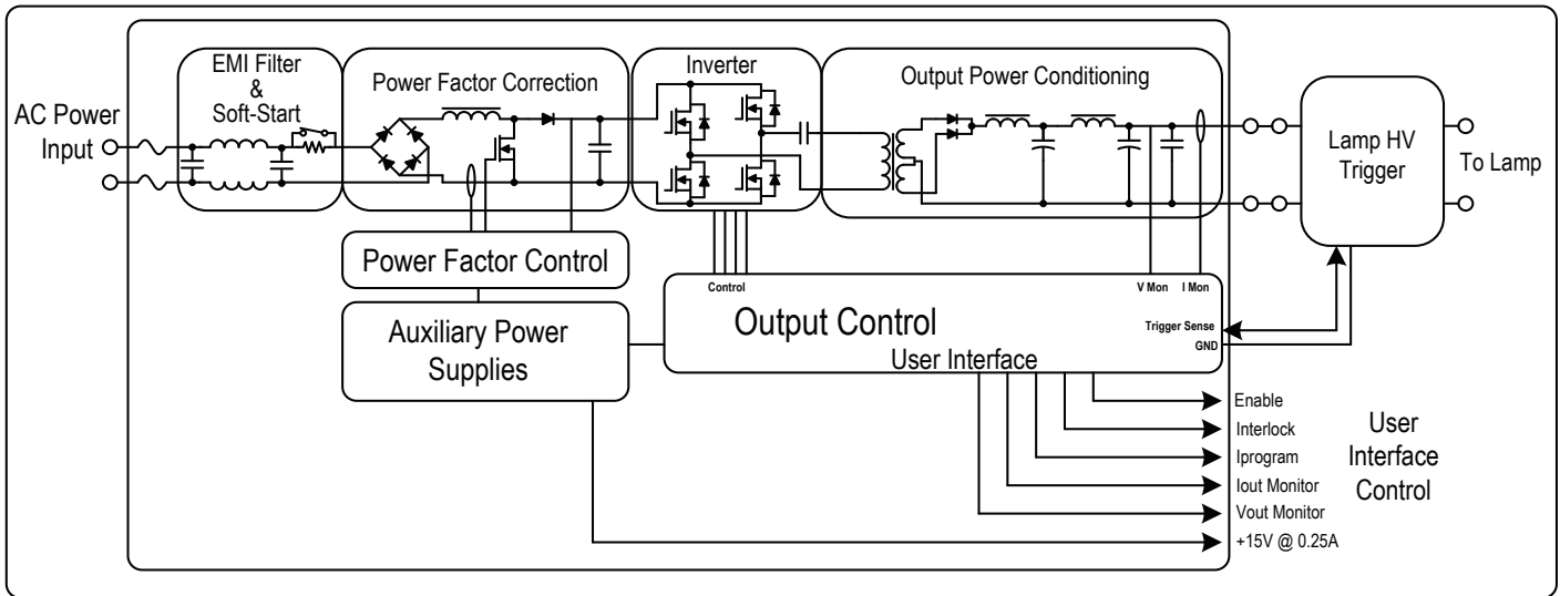
Figure 1 Block Diagram
