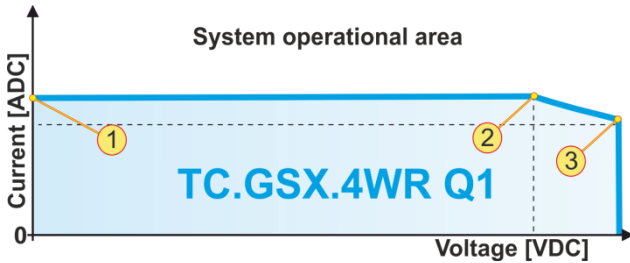
Q1 range of device TC.GSX.20.65.4WR.S.
