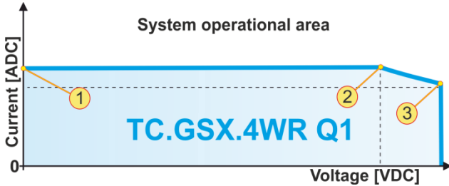
Q1 range of device TC.GSX.20.500.4WR.S.
