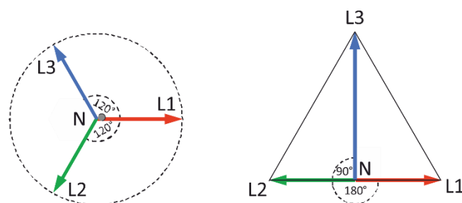
any independent phase angle possible, including split phase
