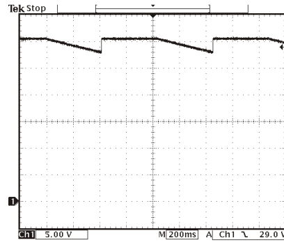
SM30-200 without Power Sink Option slow response time during voltage step down, time needed to discharge the output capacitors Trace: output voltage Voltage Programming Speed at NO LOAD
