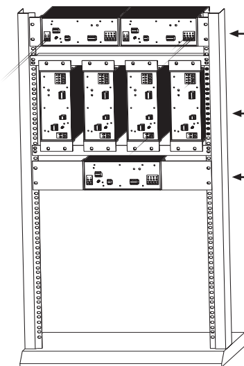
Figure 2. 19"-rack mounting
