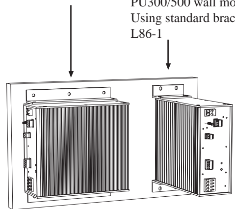
Figure 3. Wall and chassis chassis mount
