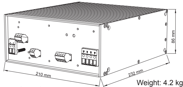
Figure 1. Dimensions
