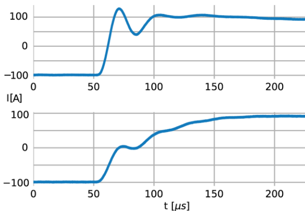
Figure 2: Parameterization example of a 36 kW, 1000 V, 108 A device: Set-value step current -97...97 A@333VDC in <50 μs with overshoot (top), in <200 μs w/o overshoot (bottom). The dynamic behavior is comparable across the series of G5 devices from low voltage to high voltage
