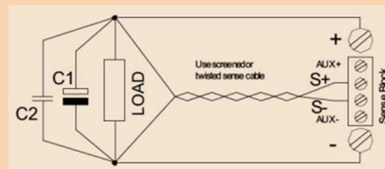
Remote Sensing (twist wires)
