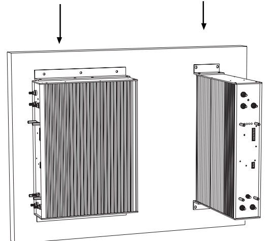
Figure 3. Wall and chassis mount.
