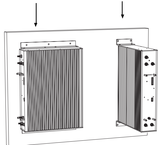
Figure 3. Wall and chassis mount.
